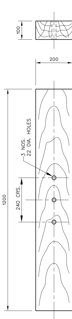
LV & 11kV POLE FOUNDATION & STAY FOUNDATION BAULK ( CLP STOCK NO. 334-240 )
