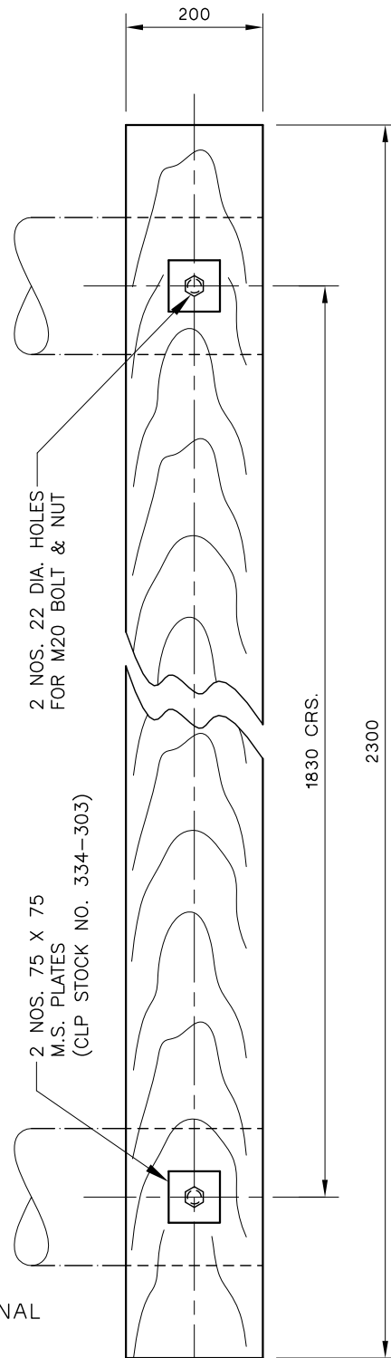
11kV TRANSFORMER 'H' POLE FOUNDATION BAULK ( CLP STOCK NO. 334-241 )
